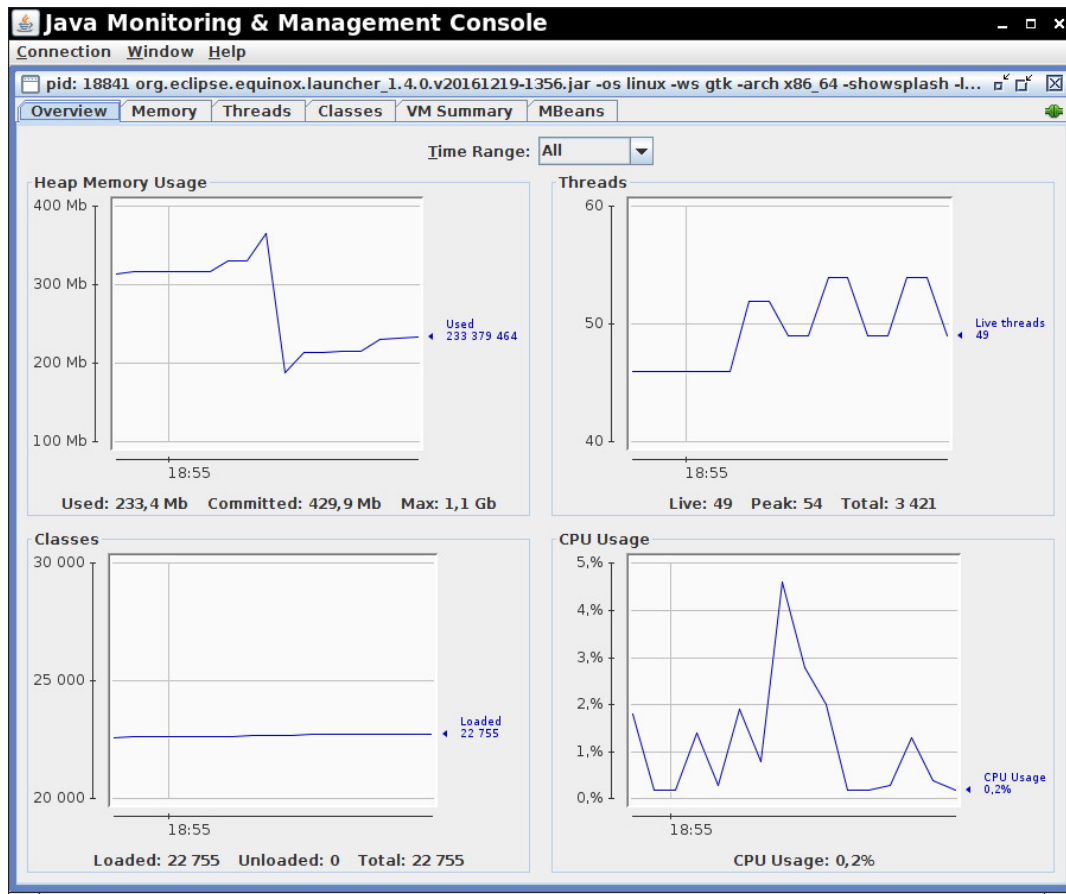
Figure 7.2: The jconsole program
