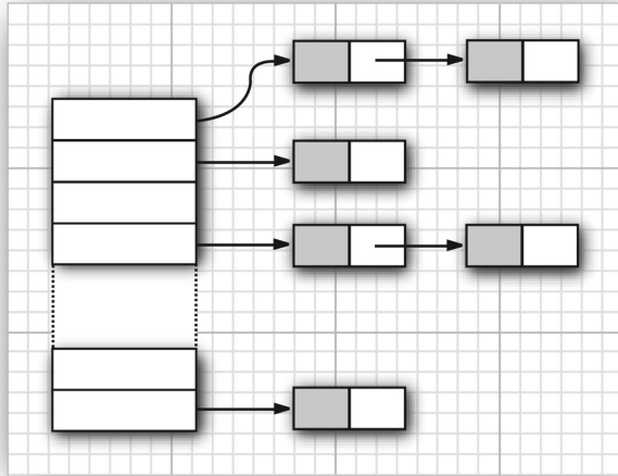
Figure 9.10: A hash table
